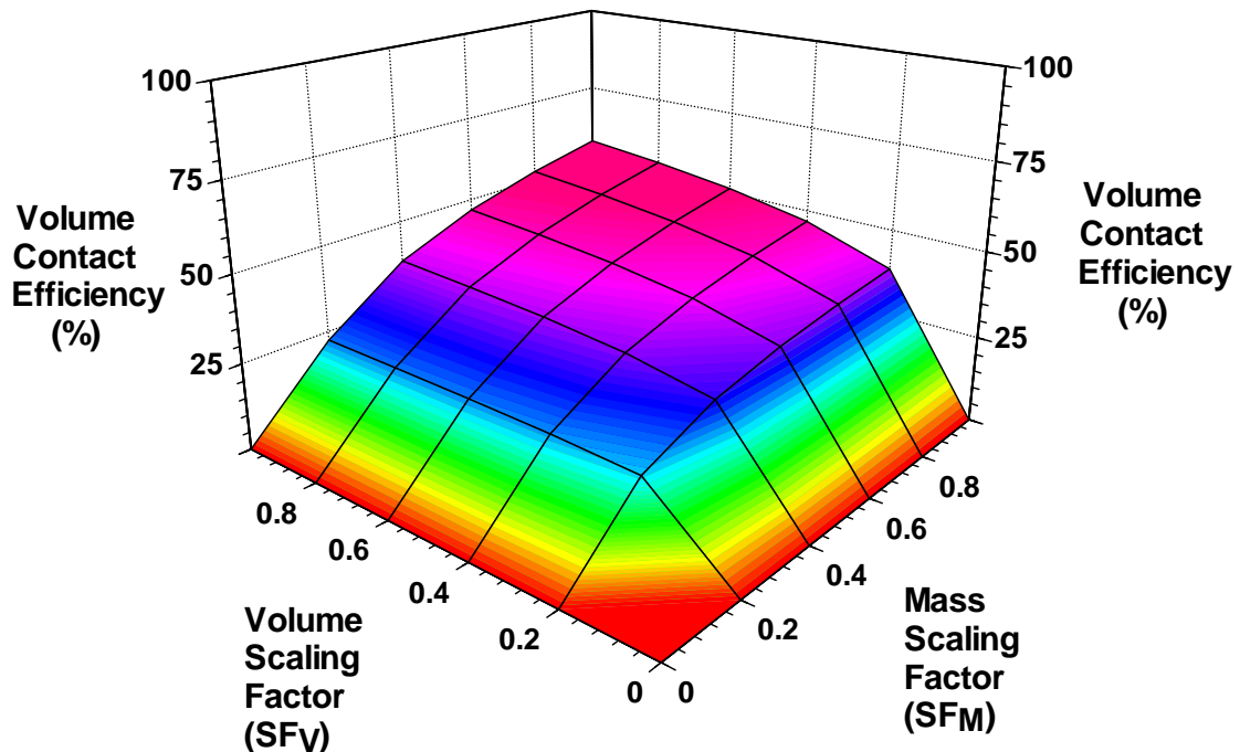
Figure 2.12 Effect of Volume Scaling Factor (SF v ) and Mass Scaling Factor (SF m ) on Volume Contact Efficiency (E v for OR \geq 0.05 OR_M ) for a Moderately Heterogeneous Aquifer with Row Spacing Equal to Approximately Two Times Well Spacing.
