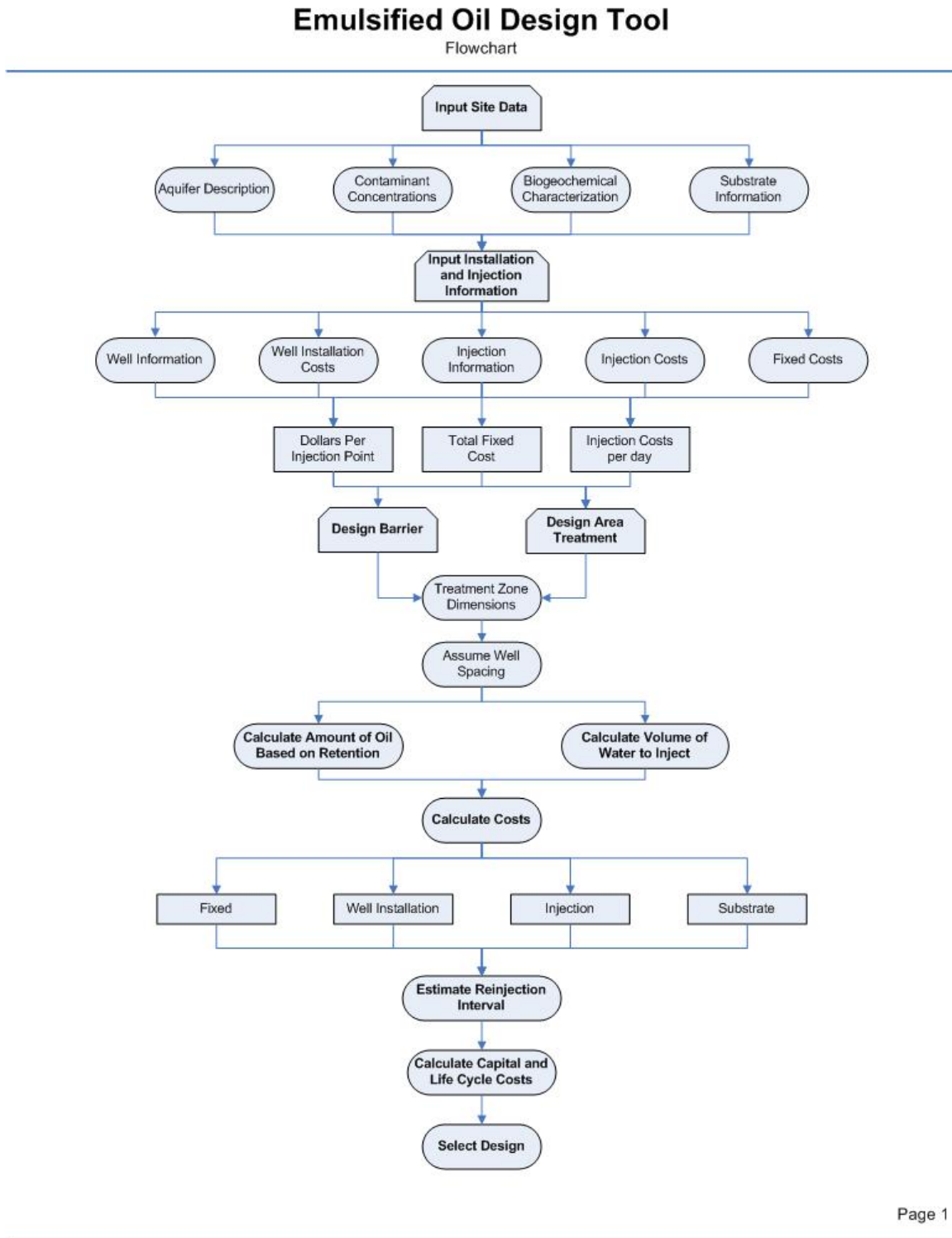
Figure 3.5. Flow Chart of the Design Process for Distributing Emulsified Oil.
